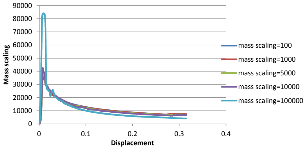
Fig13. Comparison of load-displacement diagram carried out with different values of mass scaling
